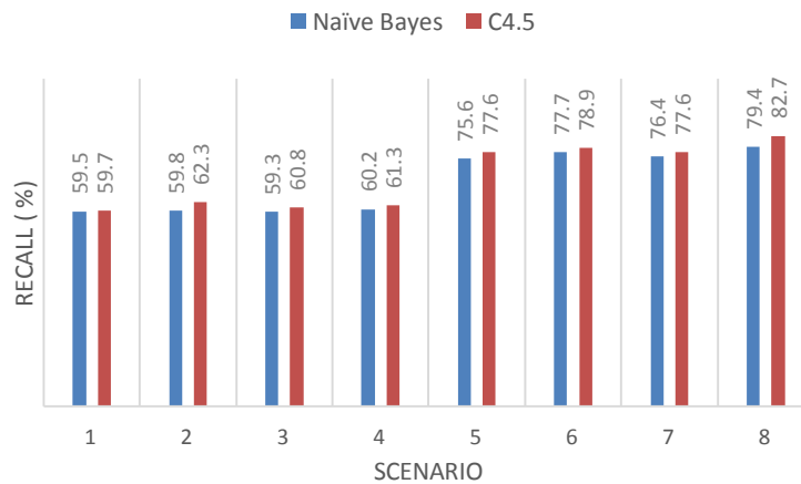
Fig. 3. Recall comparison
